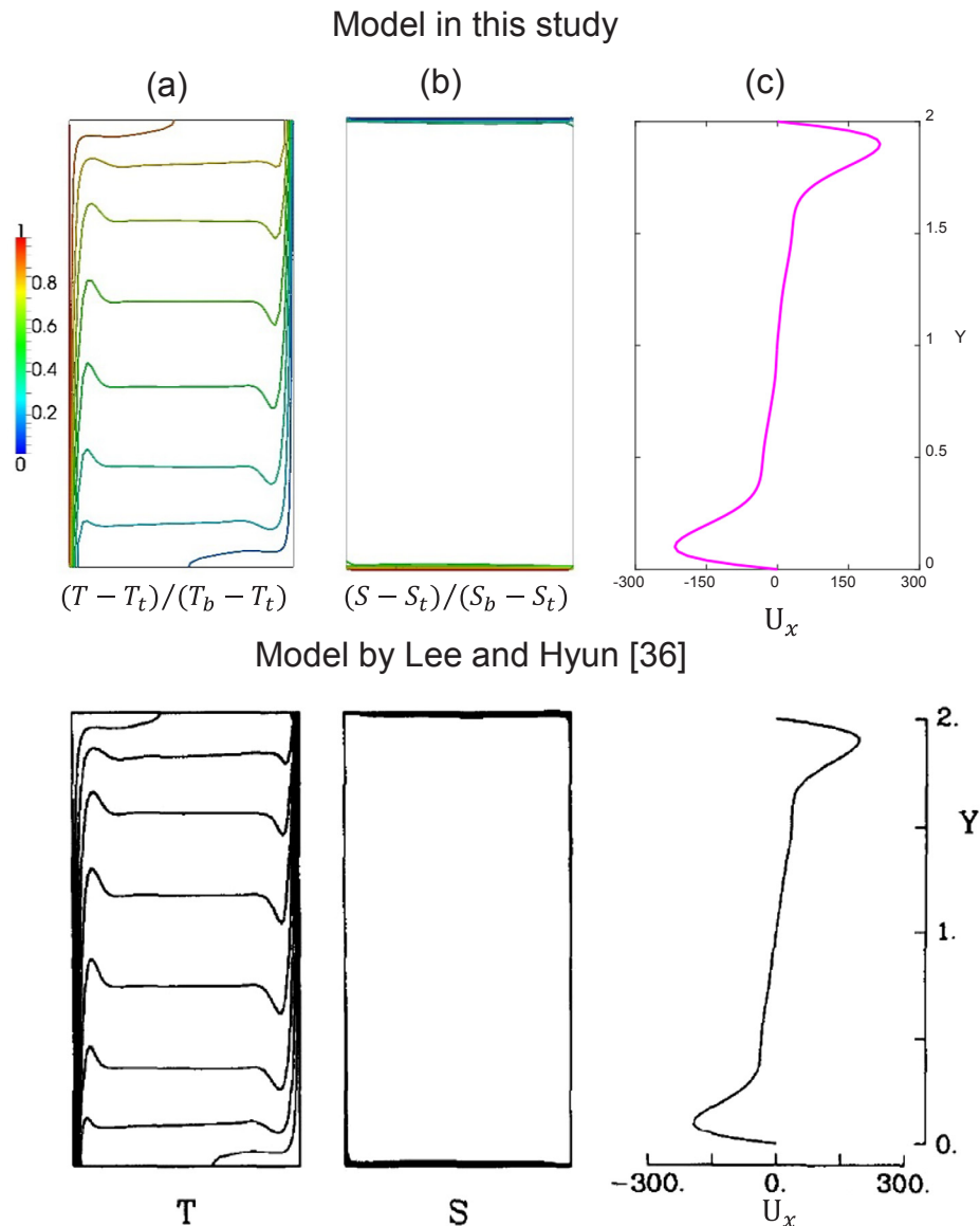
Fig. 2. Comparisons between the results from the model in the current study and the numerical results from Lee and Hyun [36]: (a) dimensionless temperature contour, (b) dimensionless salinity contour, and (c) dimensionless horizontal velocity vs dimensionless vertical axis.
